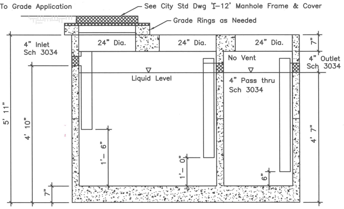
Section View
